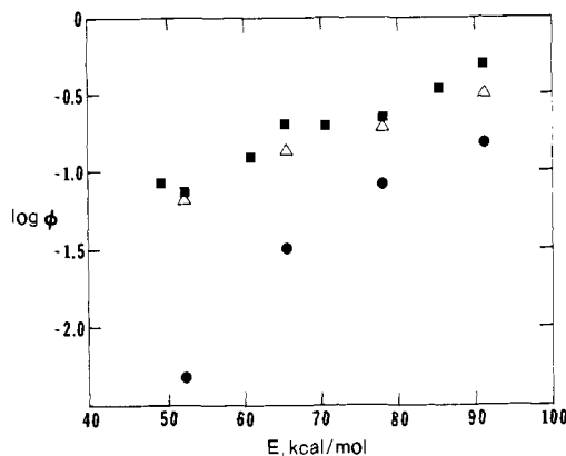
Figure 3. Plot of the log of the substitution quantum yields versus excitation energy for \text{Fe}(\text{CO})_3(\text{N}_4\text{Me}_2) (■), \text{Fe}(\text{CO})_2(\text{PPh}_3)(\text{N}_4\text{Me}_2) (●), and \text{Fe}(\text{CO})_3(\text{DAB}) (Δ).
