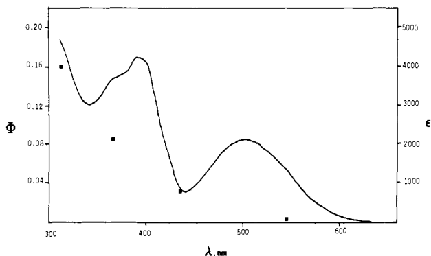
Figure 4. Quantum yields for the photosubstitution reaction \text{Fe}(\text{CO})_2(\text{PPh}_3)(\text{N}_4\text{Me}_2) + \text{PPh}_3 \rightarrow \text{Fe}(\text{CO})(\text{PPh}_3)_2(\text{N}_4\text{Me}_2) + \text{CO} , plotted vs. wavelength, along with the absorption spectrum of the reactant.
