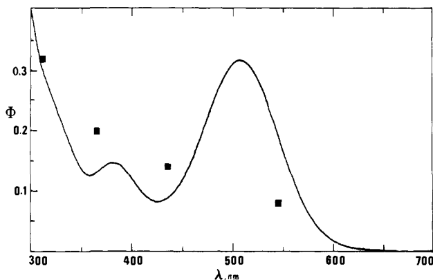
Figure 6. Quantum yields for the photosubstitution reaction \text{Fe}(\text{CO})_3(\text{DAB}) + \text{PPh}_3 \rightarrow \text{Fe}(\text{CO})_2(\text{PPh}_3)(\text{DAB}) + \text{CO} , plotted vs. wavelength, along with the absorption spectrum of the reactant.
